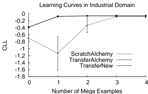
Figure 2. Accuracy on CLL
