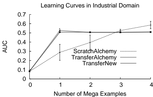
Figure 3. Accuracy on AUC
